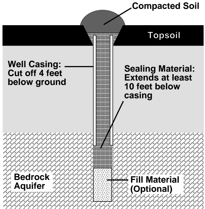
Figure 3. Placement of plugging materials in Class II wells tapping a single bedrock aquifer.
