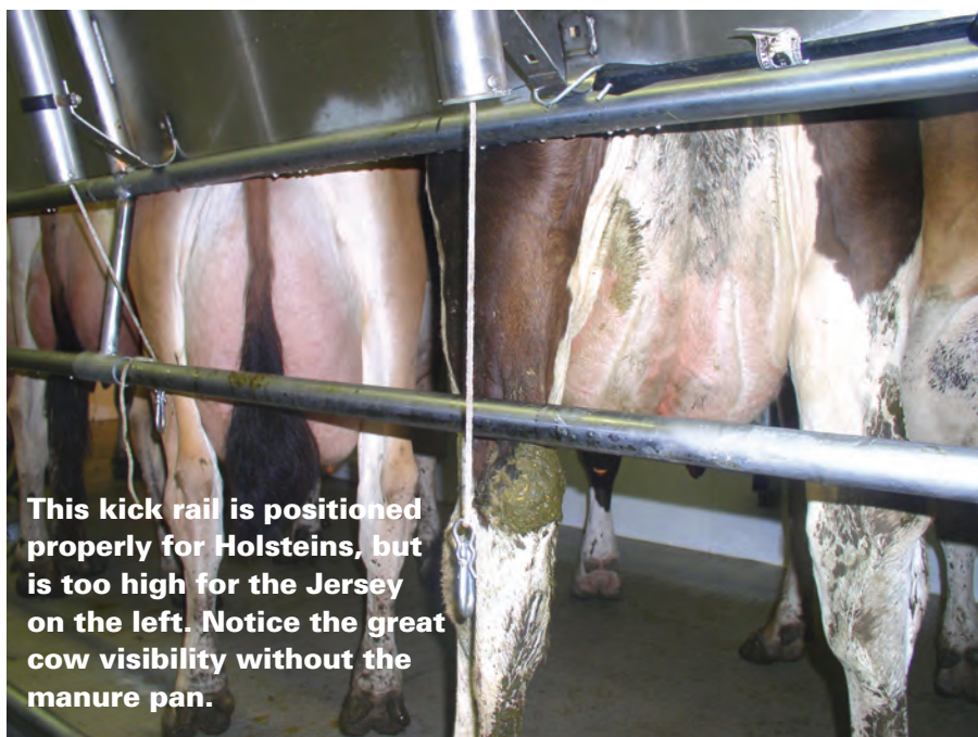
This swing 16 TRANS Iowa parlor uses galvanized steel, a floor-mounted brisket rail, and swing arm take-offs.
