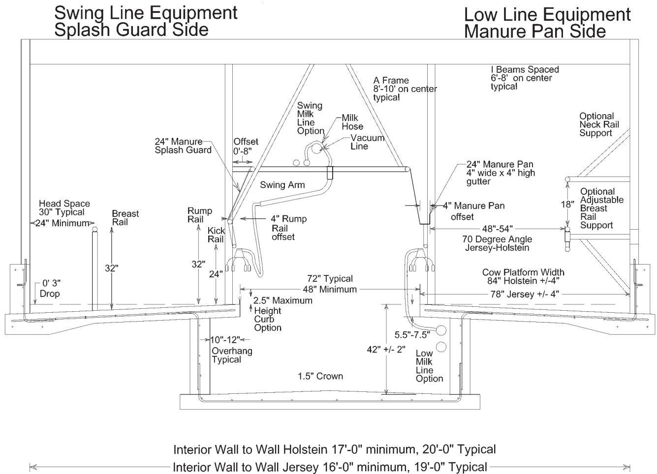
Figure 2. TRANS Iowa low-cost parlor cross section 1
