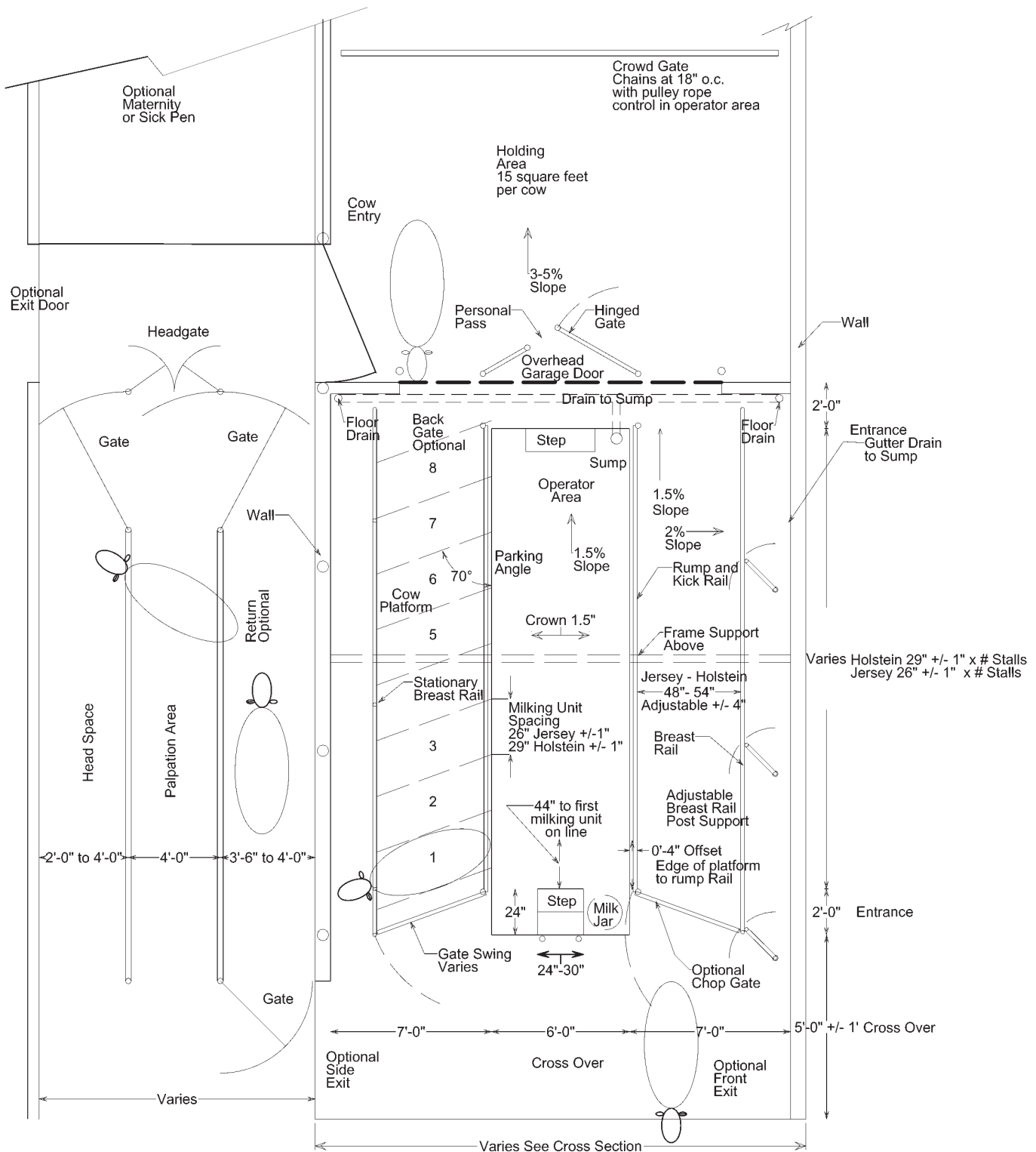
Figure 1. TRANS Iowa low-cost parlor plan 1
